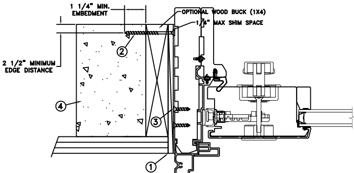
FRAME JAMB SECTION (TYP) HORIZONTAL SECTION
